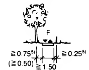
⑤ Separate footpath
